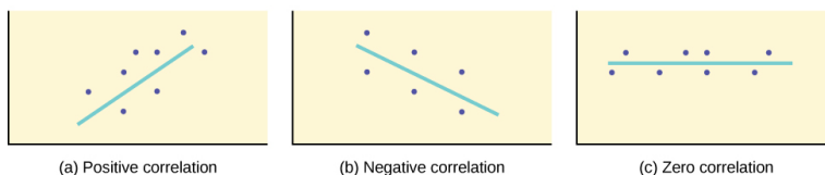
Figure 12.10 (a) A scatter plot showing data with a positive correlation: 0 < r < 1 . (b) A scatter plot showing data with a negative correlation: -1 < r < 0 . (c) A scatter plot showing data with zero correlation: r = 0 .
