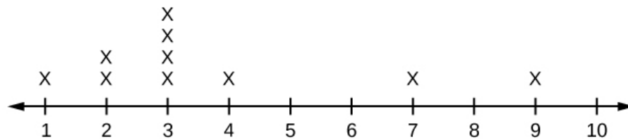
a. Figure 2.21 Terry's distribution has a right (positive) skew.
