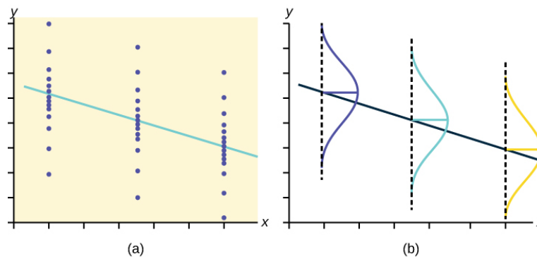
Figure 12.14 The y values for each x value are normally distributed about the line with the same standard deviation. For each x value, the mean of the y values lies on the regression line. More y values lie near the line than are scattered farther away from the line.
