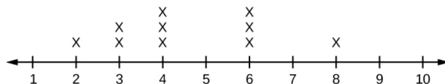
Figure 2.23 Maris's distribution is symmetrically shaped.
