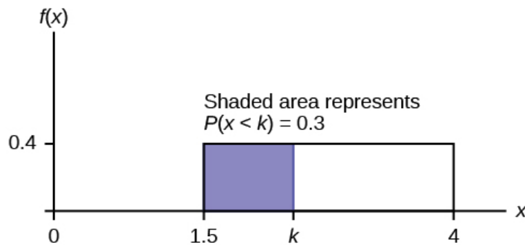
Figure 5.20 Uniform distribution between 1.5 and 4 with an area of 0.30 shaded to the left, representing the shortest 30 percent of repair times.
