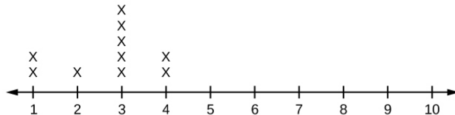
Figure 2.22 Davis's distribution has a left (negative) skew.
