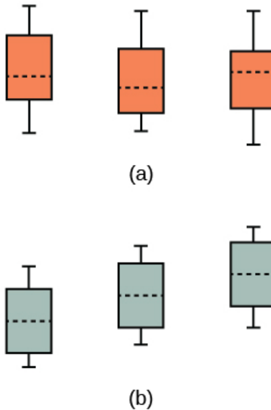
Figure 13.2 (a) We fail to reject H_0 as it may be true. All the means are about the same; the differences may be due to random variation. (b) We reject H_0 as all the means are not the same; the differences are too large to be due to random variation.
