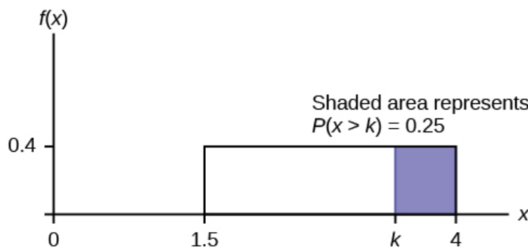
Figure 5.21 Uniform distribution between 1.5 and 4 with an area of 0.25 shaded to the right representing the longest 25 percent of repair times.
